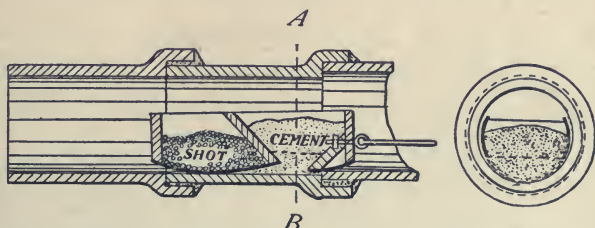
FIG. 10.—INVERT-FORMER.
